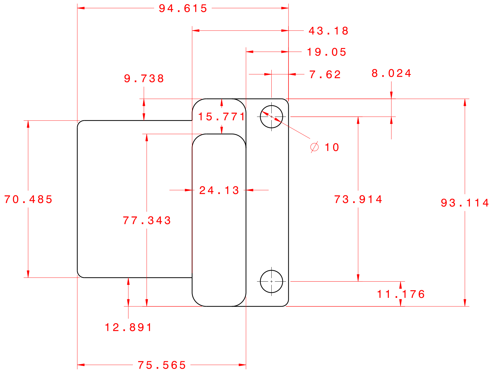
Dimensions in millimeters
